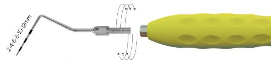
150T Probe CP 2 2-4-6-8-10-12mm
